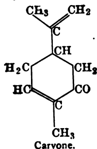
Carvone.
